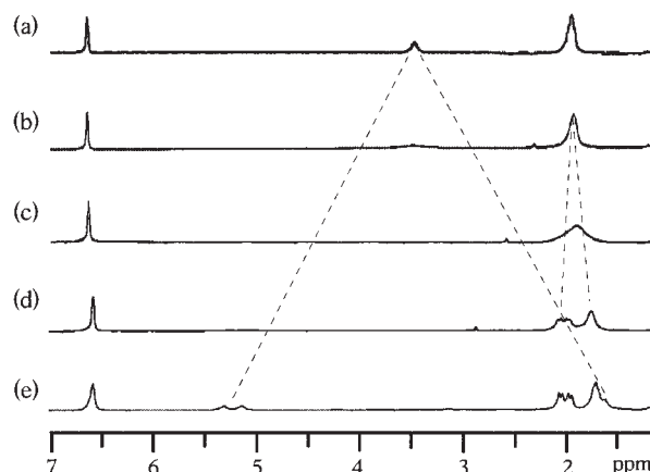
Fig. 6. ^1\text{H} NMR spectra of [\text{Pt}(\text{SeO}_3)(\text{BbtMe}_2\text{P})_2] ( 11 ) measured in \text{CDCl}_3 at (a) 25^\circ\text{C} , (b) 0^\circ\text{C} , (c) -20^\circ\text{C} , (d) -40^\circ\text{C} , and (e) -60^\circ\text{C} .
