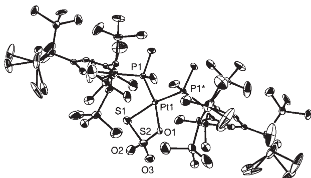
Fig. 5. ORTEP drawing of [\text{Pt}(\text{S}_2\text{O}_3)(\text{BbtMe}_2\text{P})_2] ( 8 ) with thermal ellipsoid plots (50% probability). Selected bond lengths (Å) and angles (°): Pt1–O1 2.21(3), Pt1–P1 2.263(16), P1–S1 2.312(16), O1–S2 1.54(3), S1–S2 2.079(13), S2–O2 1.43(2), S2–O3 1.43(2); P1–Pt1–P1* 105.4(2), O1–Pt1–S1 77.3(6), Pt1–O1–S2 98.1(15), Pt1–S1–S2 81.3(5), O1–S2–S1 101.4(10).
