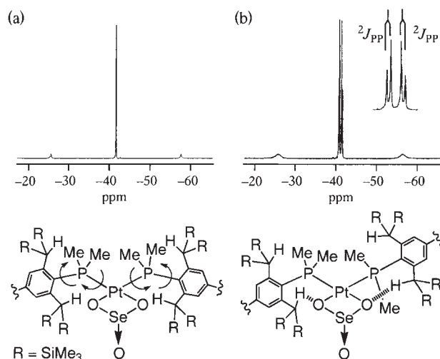
Fig. 7. ^{31}\text{P} NMR spectra of [\text{Pt}(\text{SeO}_3)(\text{BbtMe}_2\text{P})_2] ( 11 ) measured in \text{CDCl}_3 and proposed rotational behavior at (a) 25 °C and (b) -60 °C.
