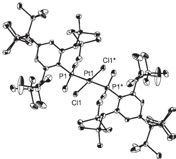
Fig. 1. ORTEP drawing of [\text{PtCl}_2(\text{BbtMe}_2\text{P})_2] ( 2b ) with thermal ellipsoid plots (50% probability). Selected bond lengths (Å) and angles (°): Pt1–Cl1 2.306(3), Pt1–P1 2.313(3); Cl1–Pt1–P1 87.15(9), Cl1–Pt1–P1* 92.85(9).
