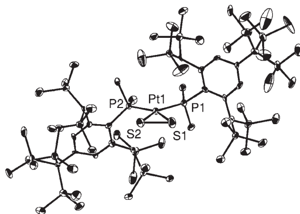
Fig. 2. ORTEP drawing of [\text{Pt}(\text{S}_2)(\text{BbtMe}_2\text{P})_2] ( 4b ) with thermal ellipsoid plots (50% probability). Selected bond lengths (Å) and angles (°): Pt1–S1 2.348(3), Pt1–S2 2.337(3), S1–S2 2.077(3), Pt1–P1 2.271(2), Pt1–P2 2.265(3); S1–Pt1–S2 52.63(9), Pt1–S1–S2 63.41(11), Pt1–S2–S1 63.96(11), P1–Pt1–S1 102.07(9), P2–Pt1–S2 98.47(9), P1–Pt1–P2 106.87(8).
