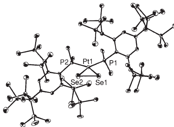
Fig. 3. ORTEP drawing of [\text{Pt}(\text{Se}_2)(\text{BbtMe}_2\text{P})_2] ( 5b ) with thermal ellipsoid plots (50% probability). Selected bond lengths (Å) and angles (°): Pt1–Se1 2.4491(10), Pt1–Se2 2.4658(10), Se1–Se2 2.3363(11), Pt1–P1 2.271(2), Pt1–P2 2.261(2); Se1–Pt1–Se2 56.76(3), Pt1–Se1–Se2 61.98(3), Pt1–Se2–Se1 61.26(3), P1–Pt1–Se1 95.44(6), P2–Pt1–Se2 99.94(6), P1–Pt1–P2 107.85(7).
